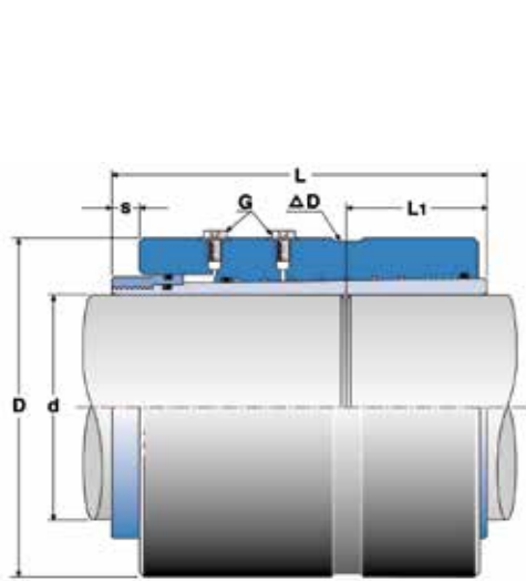
ETP HYCON® S Shaft-Shaft coupling
