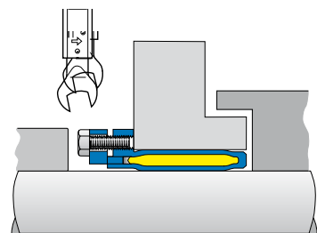
Torque wrenches for ETP-TECHNO.
