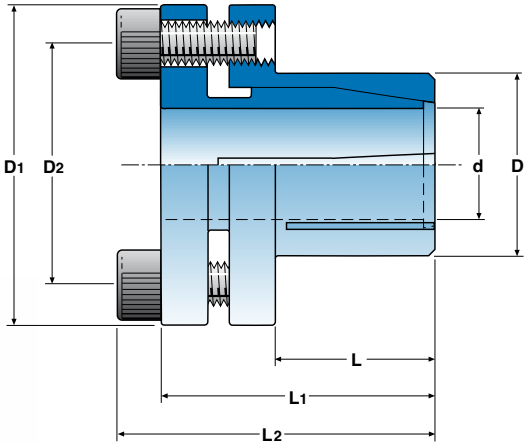
Notation: ETP-MINI XX
